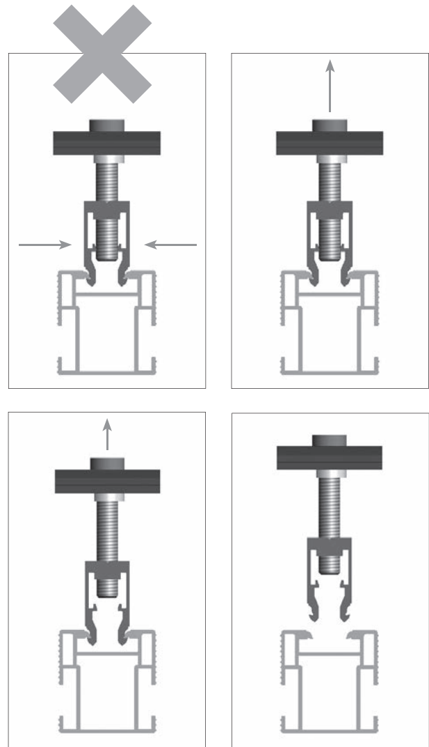
Image 7-2 Demounting steps
