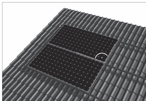
Image 8.2.-7 Landscape Installation
