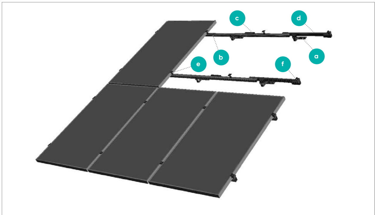
Image 2.1-1 Portrait Installation
